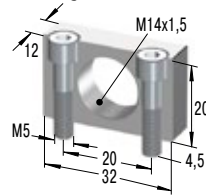
MB14SC2-V4A Montageblock
