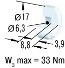
PP225 Nylonkopf
