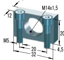
MB14SC2 Montageblock
